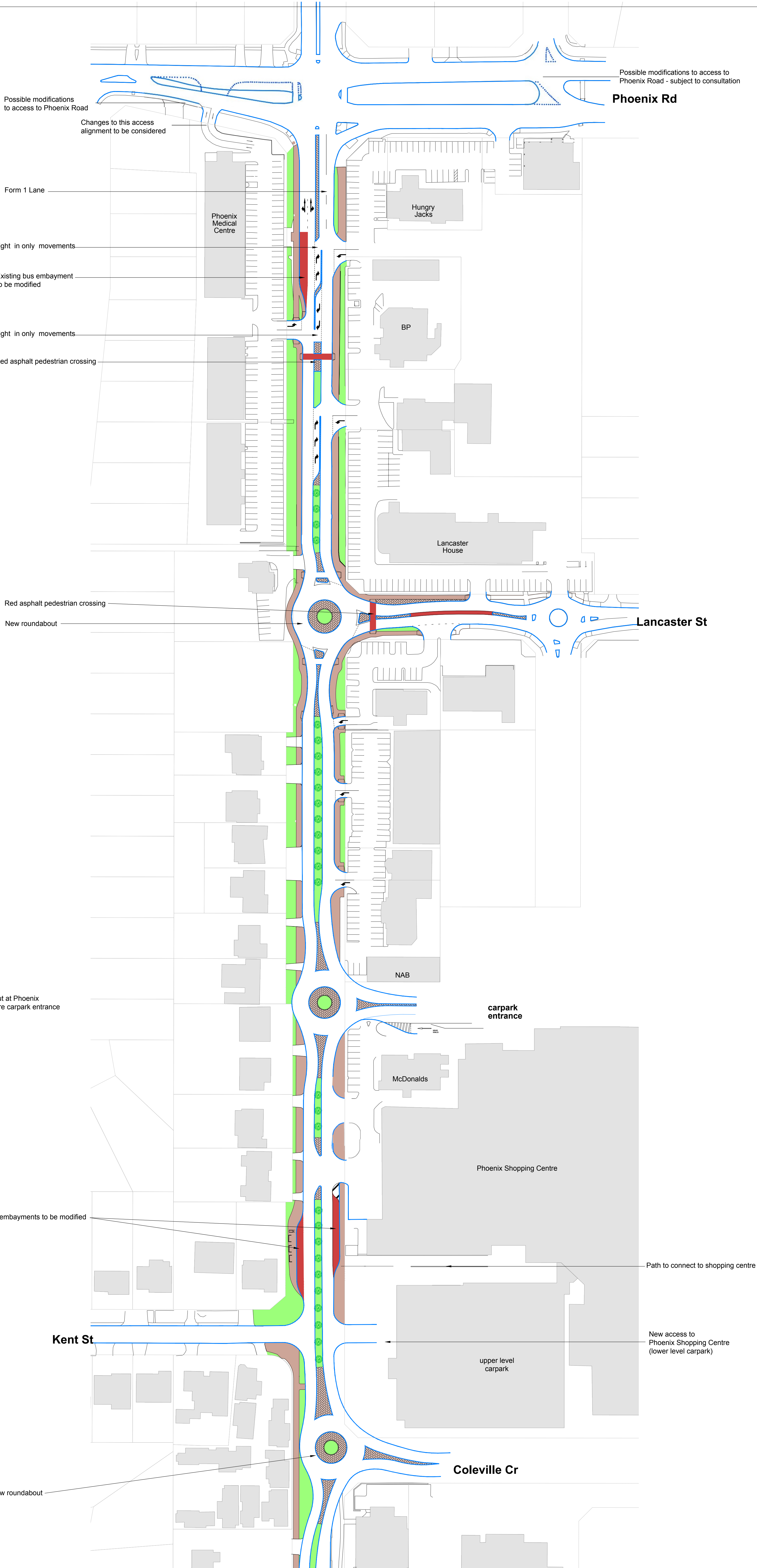
Proposed Concept Plan - Option 2 Rockingham Road, Spearwood
